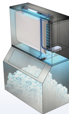
B. Mount over ice collection bin (ideal second Ice UV lamp location) use with optional interlock switch
